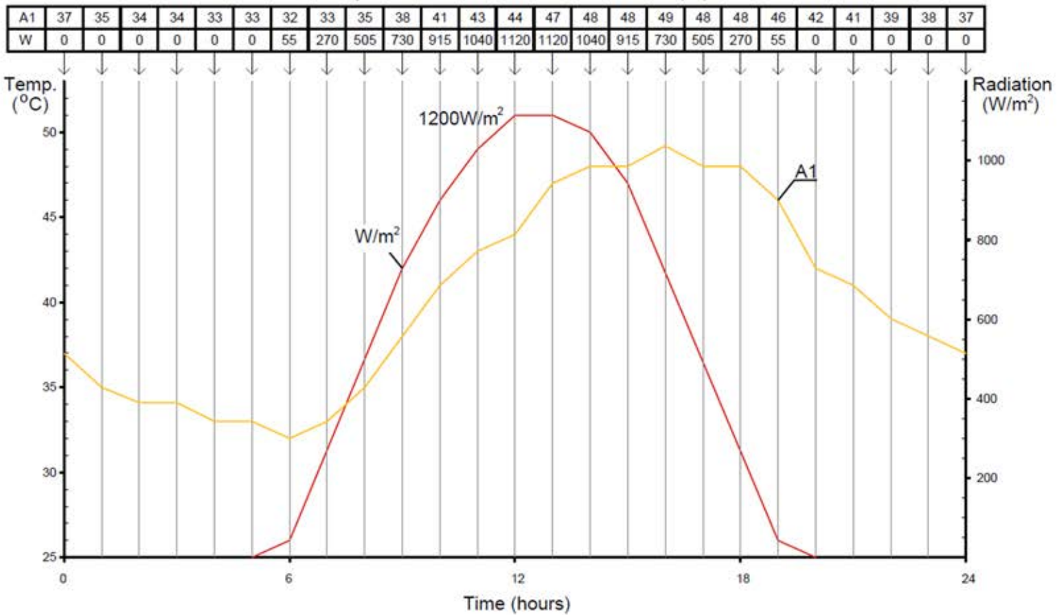
Temperatures of A1 in °C, Solar Radiation (W) in W/m 2
